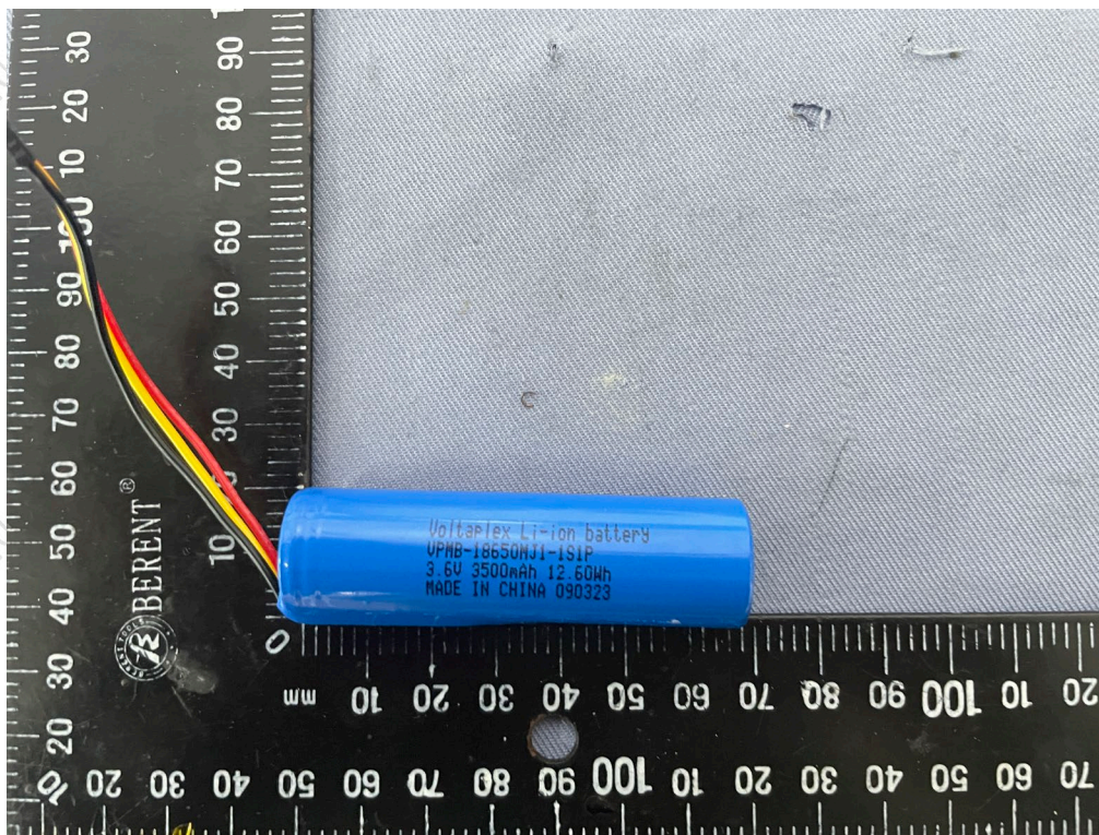
Figure 1 Overall view of battery (电池图 I)
